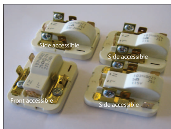
Fig.1 PTC starting devices with front and side accessible screw connections
