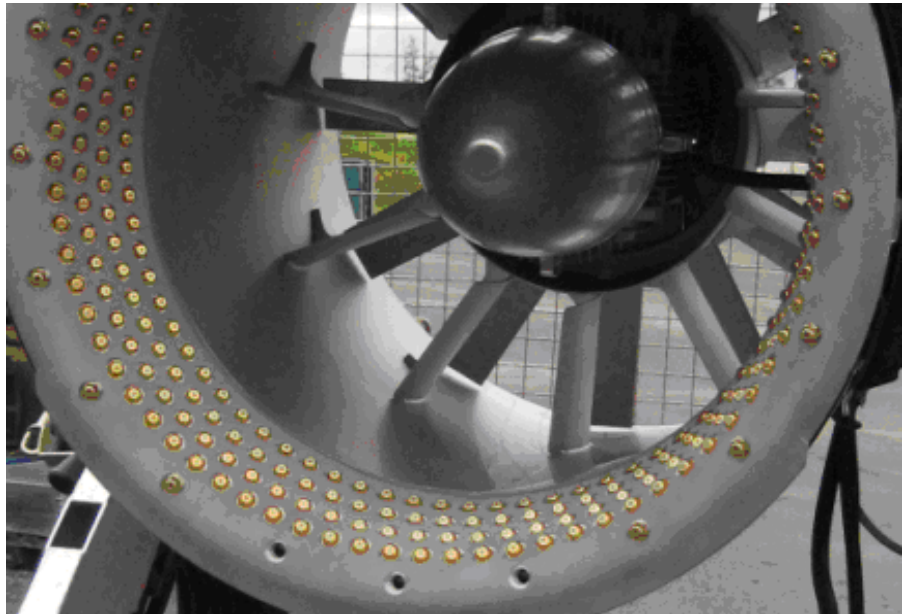
The snow canons spray pressured water out through a set of nozzles. The thin water particles formed in the air are then pushed forward by an air fan.
