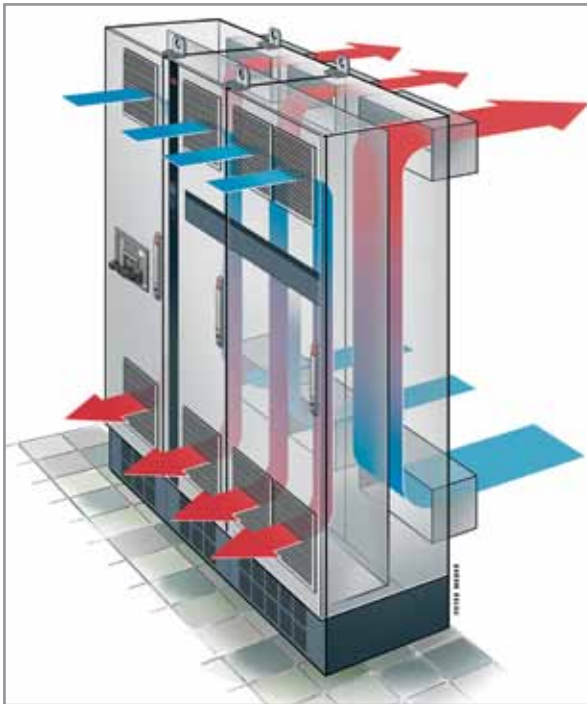
The back channel cooling system of the VLT® drive
