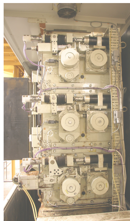
Side view of the machine. The three vertically stacked grinding units and the device for adjusting the positions of the large grinding rolls are clearly visible.
