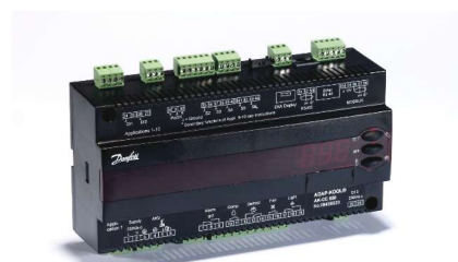
Controlling CO 2 in evaporators - AK-CC550A and AKVH, New generation of Danfoss ADAP-KOOL™ injection system for CO 2 evaporators
